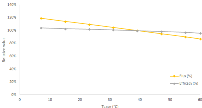
Flux and efficacy versus temperature at Tc (@U nominal)
